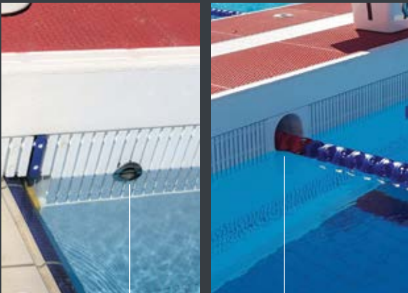
Fixed 316 stainless steel cup anchors for outside lanes Flip Down, Flip Up pivoting anchor: - 316 stainless steel anchoring plate - included on both sides
